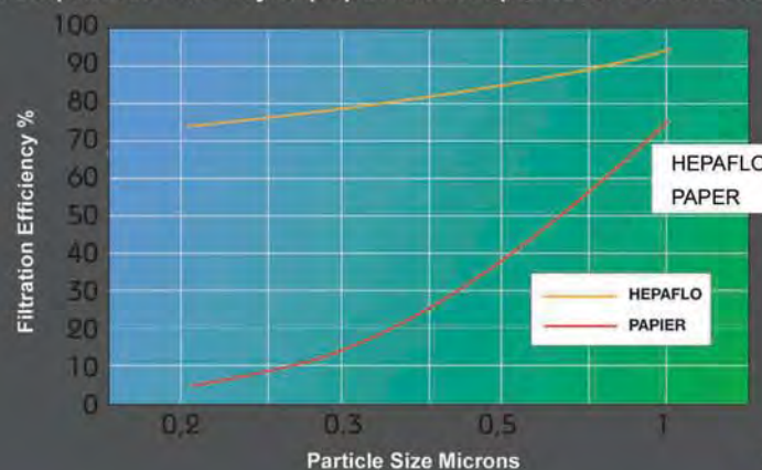
Comparison of 2 layer paper and HepaFlo filtration efficiency.
